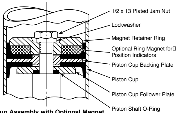
Piston Cup Assembly with Optional Magnet for Valves with Position Indicators
